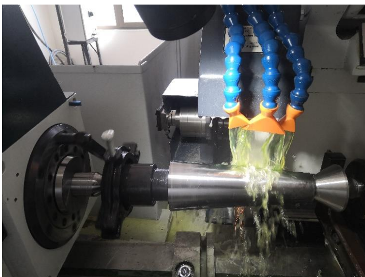
Taper Profile Grinding on Mandrels
