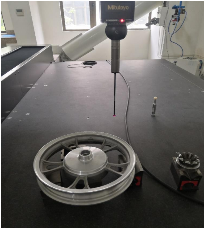
EV 2 Wheeler Alloywheel Inspection
