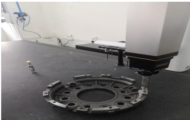
Clutch Plate Inspection
